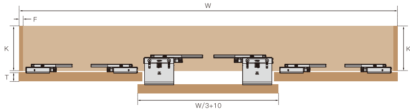
三门双缓冲 (三门带对碰) Full soft close for 3 doors
