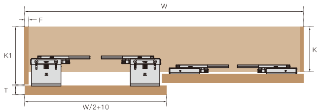
两门双缓冲 Double soft close for 2 doors
