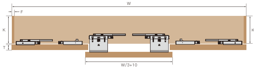
三门双缓冲 Double soft close for 3 doors
