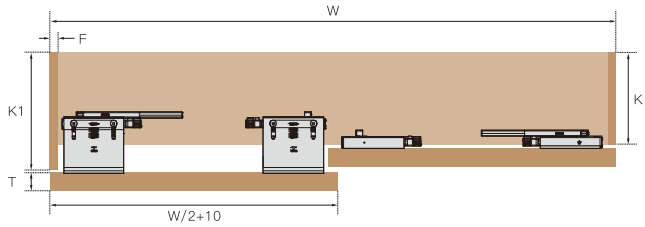
两门单缓冲 Single side soft close for 2 doors
